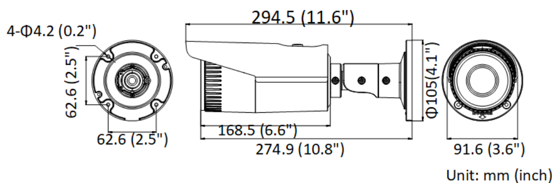
Without Junction Box
